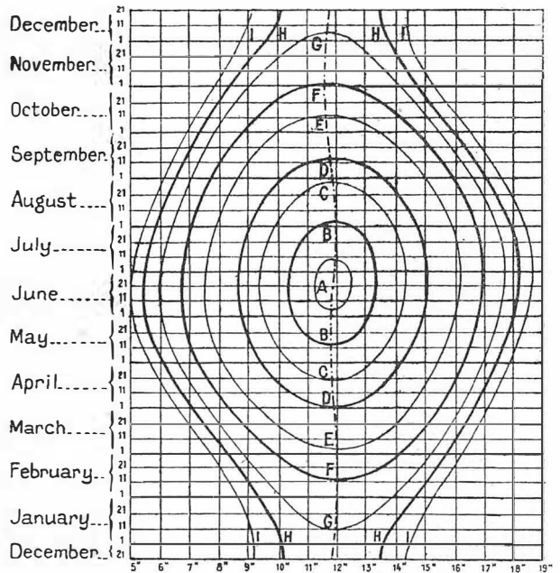
FIG. 169. CURVES OF EQUAL LIGHT-VALUES (Greenwich Mean Time)
