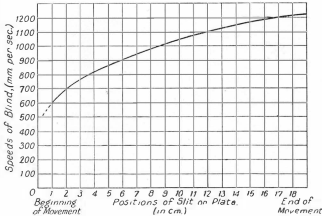
FIG. 123. VARIATION OF SPEED OF BLIND DURING EXPOSURE
