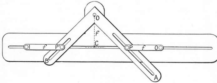
FIG. 50. SELF-FOCUSSING LINKAGE (Carpentier)
