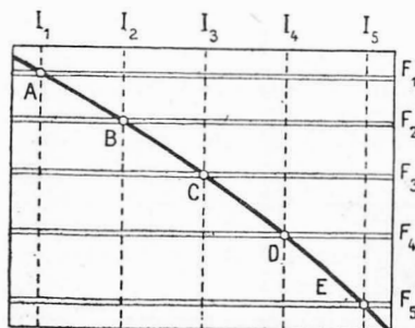
FIG. 120. ACTION OF FOCAL-PLANE SHUTTER
