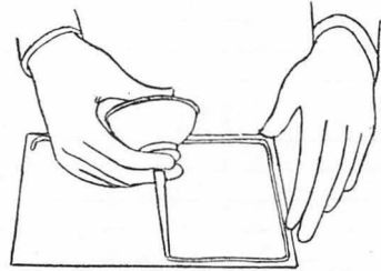
FIG. 186. EDGE MOUNTING WITH FISH-GLUE
