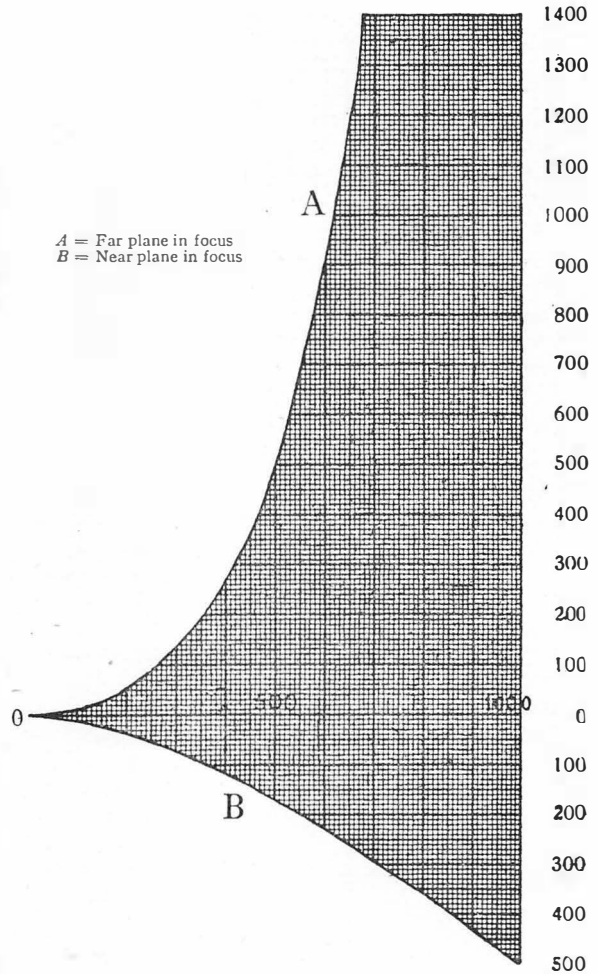
Depth of field (circle of confusion = 1/1,000 the camera extension). The unit of length is the diameter of the effective aperture
