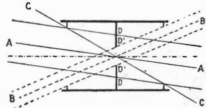
FIG. 37. CUT-OFF OF MARGINAL RAYS
