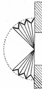
FIG. 108. BELLOWS SHUTTER
