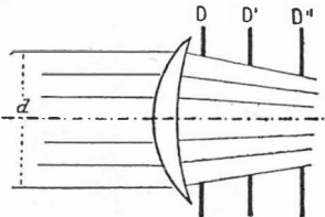
FIG. 53. EFFECTIVE APERTURE
