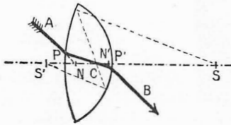
FIG. 16A. OPTICAL CENTRE IN LENS
