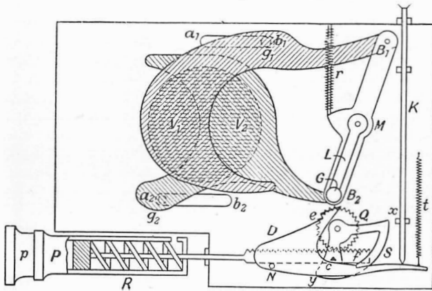
FIG. 109. DOUBLE-PLATE SHUTTER—SET
