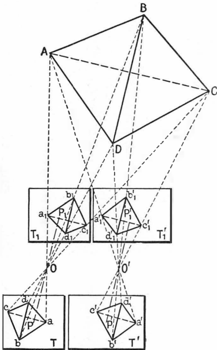
FIG. 200. OPTICS OF STEREOSCOPIC PHOTOGRAPHY
