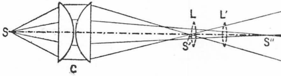
FIG. 193. EFFECT OF DISTANCE OF ENLARGING LENS FROM CONDENSER
