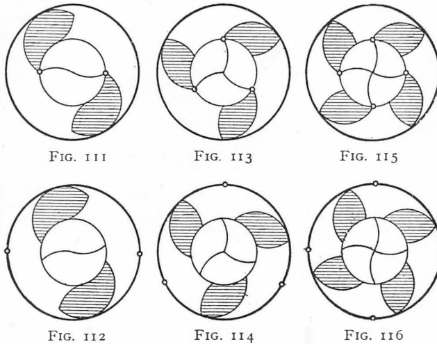
THEORETICAL FORMS OF TWO-, THREE-, AND FOUR-LEAF DIAPHRAGM SHUTTERS
