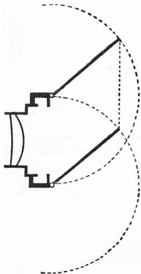
FIG. 106. DOUBLE-FLAP SHUTTER
