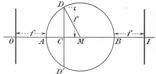
FIG. 51A. PRINCIPLE OF FOCUSSING LINKAGE.
