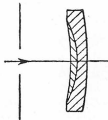
FIG. 67. GRUBB'S SINGLE LENS F/16
