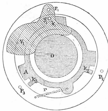
FIG. 118. COMPOUND SHUTTER, OPEN
