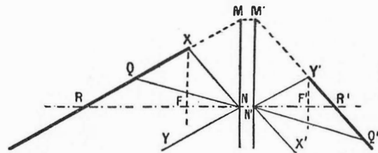
FIG. 48. IMAGE FORMATION ON INCLINED SURFACE
