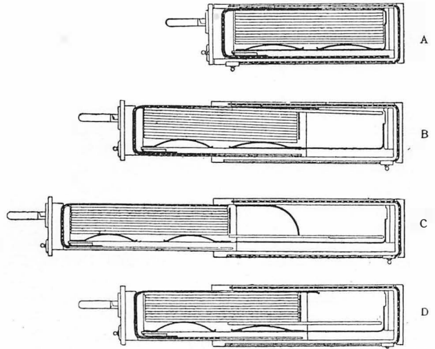
FIG. 132. OPERATION OF MAGAZINE CHANGING BOX
