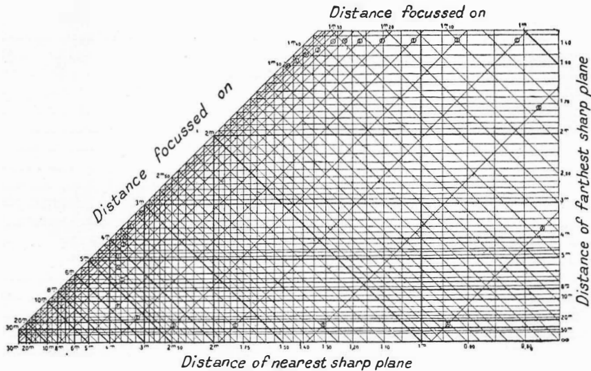
FIG. 61. CHART OF DEPTH OF FIELD
