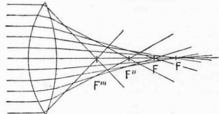
FIG. 21. SPHERICAL ABERRATION
