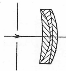
FIG. 68. DALLMEYER'S SINGLE LANDSCAPE LENS, F/11
