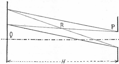
FIG. 59. GEOMETRY OF HYPERFOCAL DISTANCE
