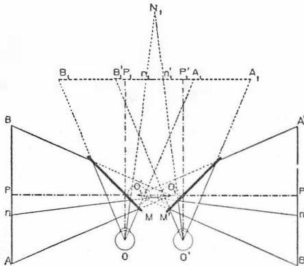
FIG. 210. WHEATSTONE STEREOSCOPE
