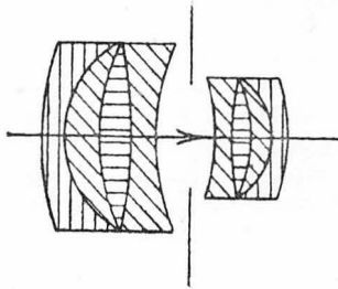
FIG. 78. RUDOLPH'S DOUBLE PROTAR, F/7.7
