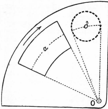
FIG. 98. ROTARY SHUTTER
