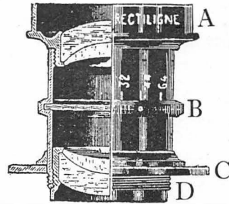
FIG. 87. PARTS OF LENS MOUNT
