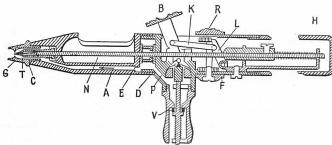
FIG. 187. MECHANISM OF AN AIR-BRUSH
