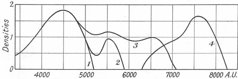
FIG. 142. CURVES OF SPECTRAL SENSITIVENESS OF EMULSIONS
