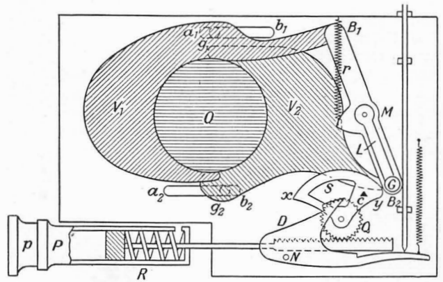
FIG. 110. DOUBLE-PLATE SHUTTER—OPEN
