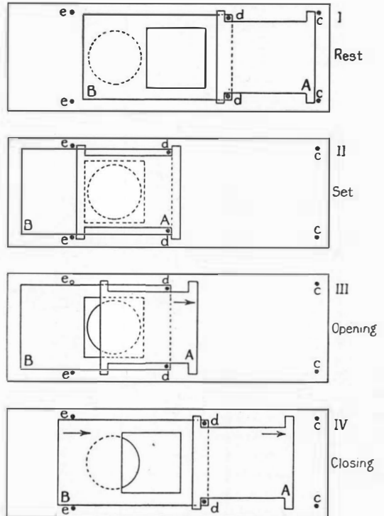
FIG. 104. ACTION OF GUILLOTINE SHUTTER
