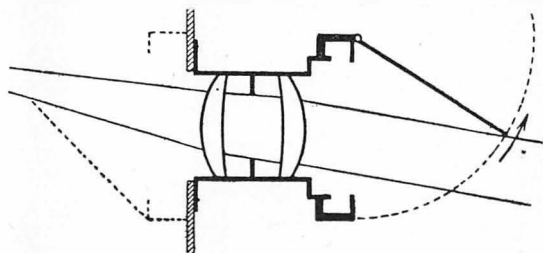
FIG. 105. GUERRY SINGLE-FLAP SHUTTER
