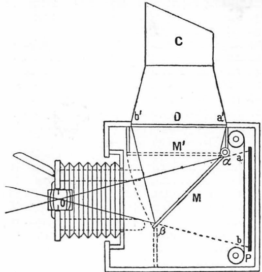
FIG. 131. REFLEX CAMERA
