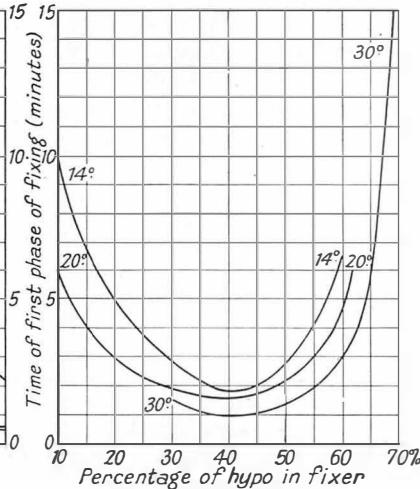
FIG. 174. VARIATION OF FIXING ACTION WITH STRENGTH OF HYPO BATH (Piper)
