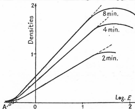
FIG. 140. CHARACTERISTIC CURVES OF A PLATE
