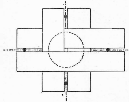
FIG. 14. MAKING THE APERTURE FOR PINHOLE PHOTOGRAPHY
