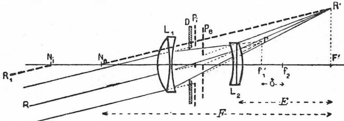
FIG. 83. OPTICS OF THE TELEPHOTO LENS
