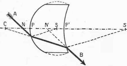
FIG. 16B. OPTICAL CENTRE OUTSIDE LENS
