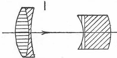
FIG. 85. FIXED-FOCUS TELEPHOTO, F/4.8 (LEE)
