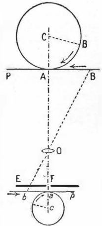
FIG. 188. COPYING ON A ROTATING SENSITIVE SURFACE
