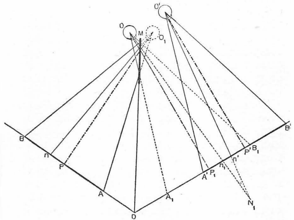
FIG. 212. SINGLE-MIRROR STEREOSCOPE (Pigeon)
