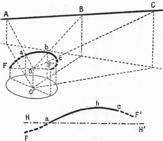
FIG. 9. PANORAMIC PERSPECTIVE
