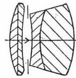
FIG. 73. STEINHEIL'S GROUP ANTIPLANAT, F/6.2
