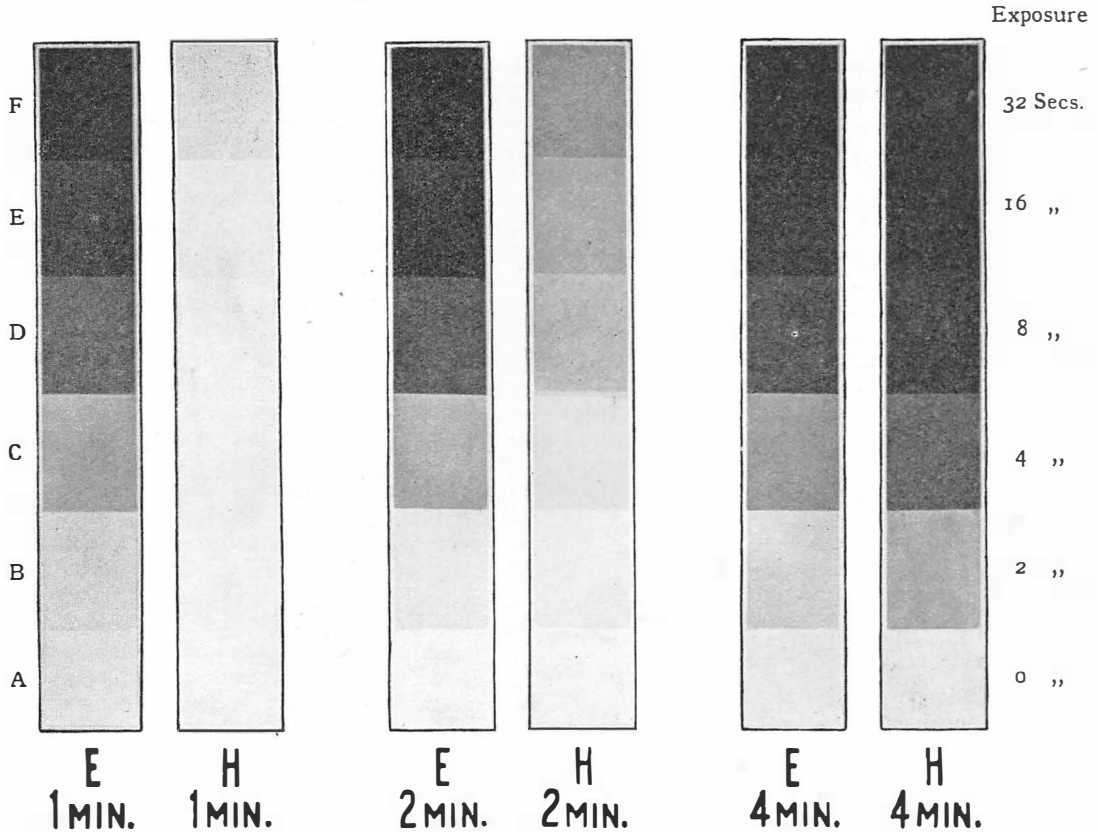
FIG. 171. COMPARATIVE EFFECTS OF METOL (E) AND HYDROQUINONE (H) DEVELOPERS
