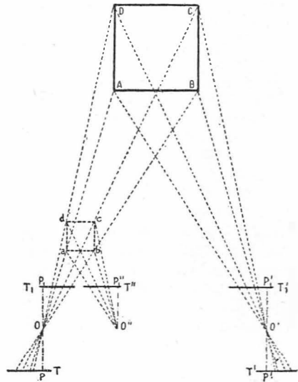
FIG. 203. STEREOSCOPY WITH WIDELY SEPARATED VIEWPOINTS
