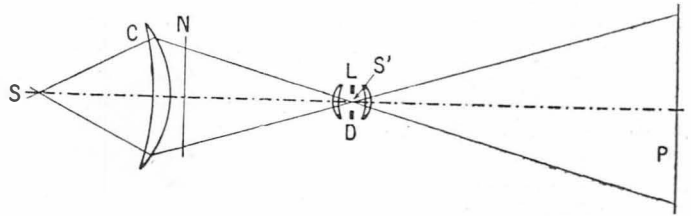
FIG. 192. IDEAL OPTICAL SYSTEM OF CONDENSER ENLARGER
