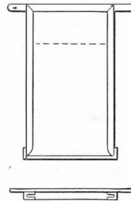
FIG. 161 DEVELOPING HANGER
