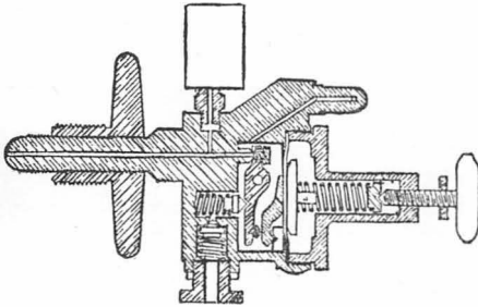
FIG. 198. REGULATOR FOR OXYGEN GAS CYLINDER
