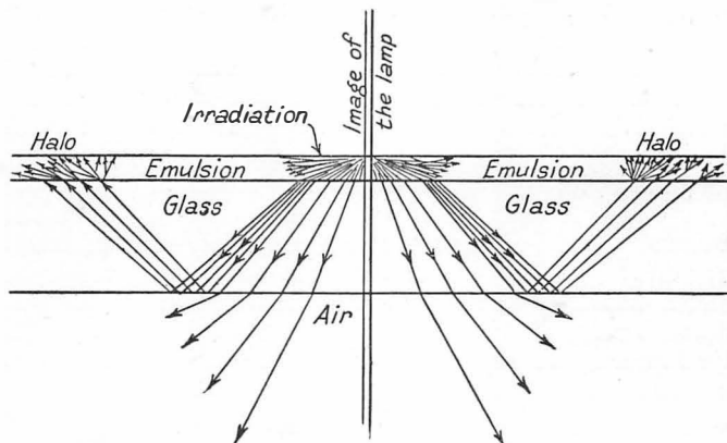
FIG. 149. MECHANISM OF HALATION
