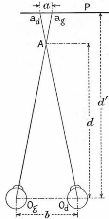
FIG. 201. ZONES IN BINOCULAR VIEWING
