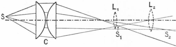
FIG. 194. EFFECT OF DECENTERING OF LIGHT-SOURCE FROM OPTICAL AXIS
