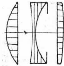
FIG. 79. TAYLOR'S COOKE LENS, F/6.5
