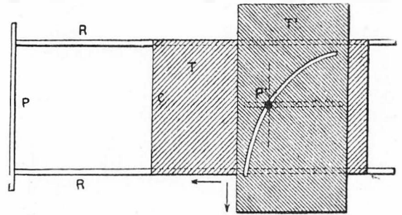
FIG. 52. CAM SELF-FOCUSsing (Pizzighelli)
