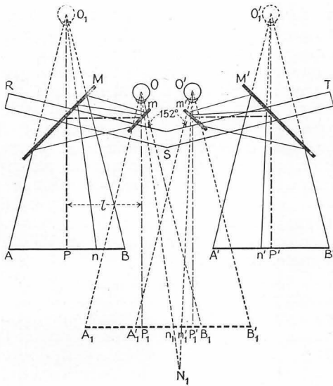
FIG. 211. TWO-MIRROR STEREOSCOPE (Cazes)
