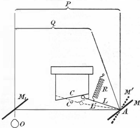
FIG. 130. DIAGRAM OF A COUPLED TELEMETER
